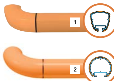
HOT-WELDED DECOCHOC Panel / panel or panel / floor hot-welding
